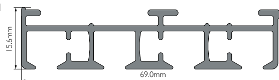
Panel Track 4-Channel Headrail 6mm Channel
