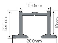
Recess M-Section Aluminium Profile Track 6mm Channel
