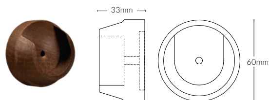
RECESS BRACKET
