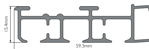
Panel Track 3-Channel Wall-fix Headrail 6mm Channel
