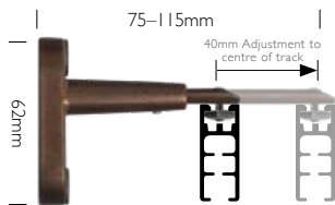
Standard Adjustable
