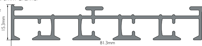
Panel Track 5-Channel Headrail 6mm Channel
