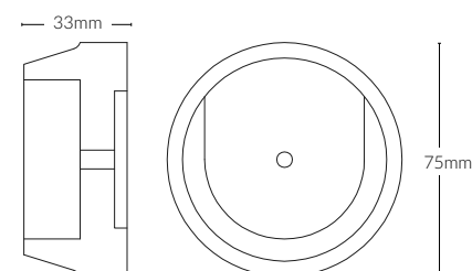
RECESS BRACKET
