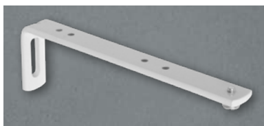
14cm L-Extension Bracket Code: 16LB141W Packed: 10 Min Qty: 10
