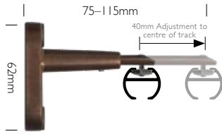
Standard Adjustable
