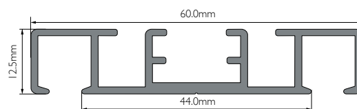
Double Project Pre-drilled ‡ Track – Ceiling Fix 6mm Channel
