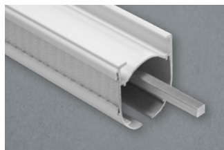
Closed Cassette System Headrail + 5mm Square Axle Bar Size: 5.8m Code: 17CLHRAX Packed: 10 Lengths Min Qty: 10
