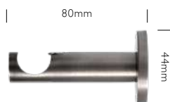
Contemporary Bracket
