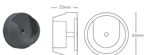
RECESS BRACKET
