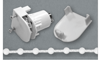
Workroom Kit Chain Housing + End Cap + 100cm Chain Chain Control: 1:2 Code: 17CQCH2C Chain Control: 1:4 Code: 17CQCH4C Packed: 10 Min Qty: 10
