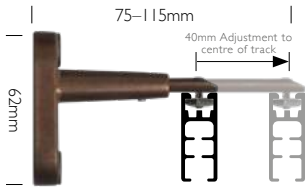
Standard Adjustable
