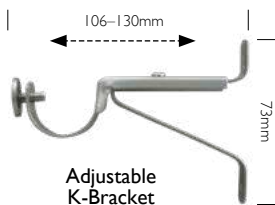
Contemporary Bracket
