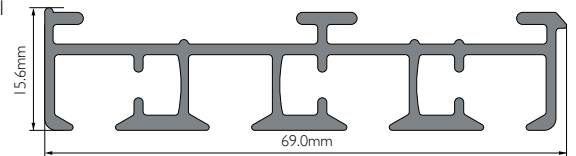
Panel Track 4-Channel Headrail 6mm Channel
