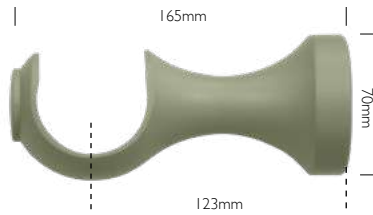
50mm Cup Bracket
