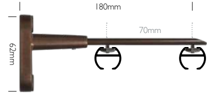
Long Adjustable – Double Use
