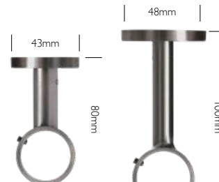
Short Ceiling Bracket
