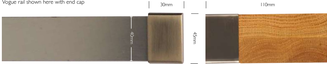
Vogue Brushed Silver Aluminium Rail Code: 16VG500E
