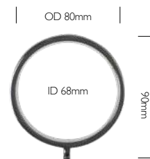
Rings Include Nylon Inserts To Ensure Quieter Running
