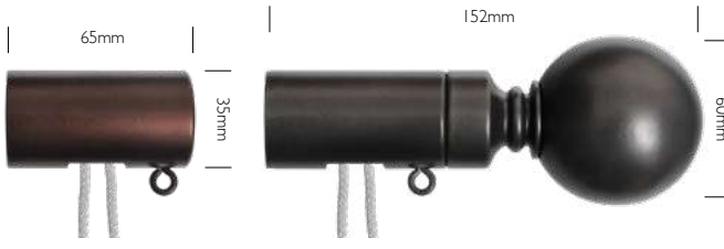
Barrel Finial – Corded as standard with Complete Kits
