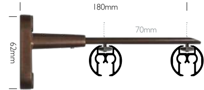
Long Adjustable – Double Use
