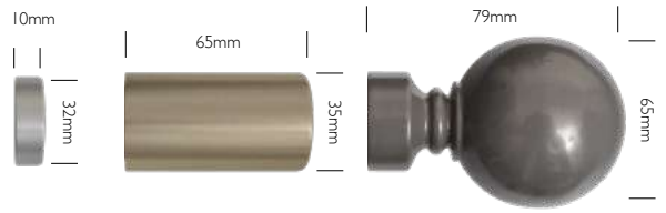
End Cap as standard with Complete Kits
