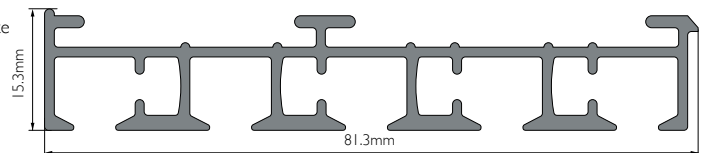
Panel Track 5-Channel Headrail 6mm Channel
