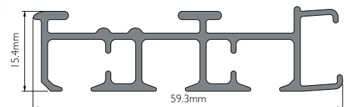
Panel Track 3-Channel Wall-fix Headrail 6mm Channel
