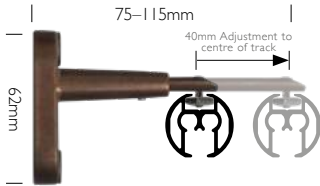
Standard Adjustable
