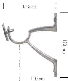
Luxury End Bracket
