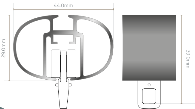
Ocular Track Profile with Roller Glider
