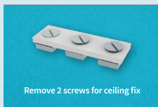
T-Join Connecting Piece Can also be used as a Ceiling Fix Bracket ○ White Code: 16HO015W ● Grey Code: 16HO015T
