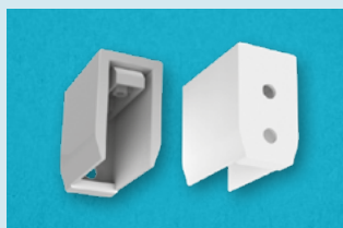
Cubicle Rail Side Bracket/End Cap (with holes) For Wall Fix ○ White Code: 16HO017W ● Grey Code: 16HO017T
